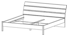
76166 King bed (US+UK) 201.1 x 227.5 x 41.5/97.1 cm 79¼ x 89½ x 16¼/38¼" Colours: 20 - 61
